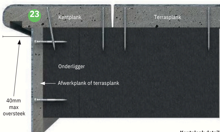
Kantplank detail
